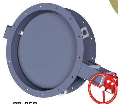
CD-95R Bubble-Tight Isolation
